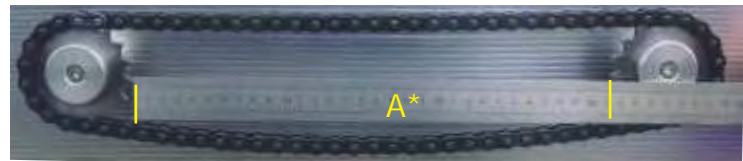
Installation and final dimensions for the ROLL-RING chain tensioner/series ISO B:
